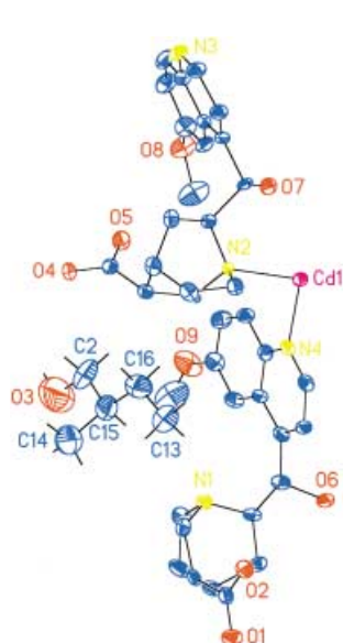
Figure 5. ORTEP view of an asymmetric unit of 3 (30% probability displacement ellipsoids). The H atoms of the frameworks are omitted for clarity.
