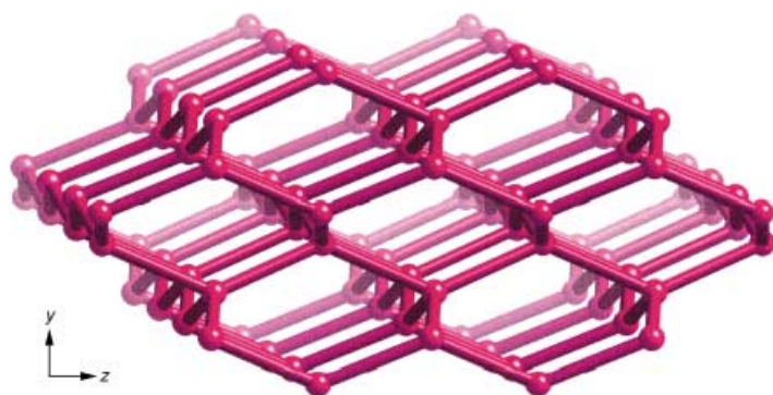
Figure 2. A topological perspective view of 1 in which the straight lines and circles represent the quinene ligands and Cd atoms, respectively.
