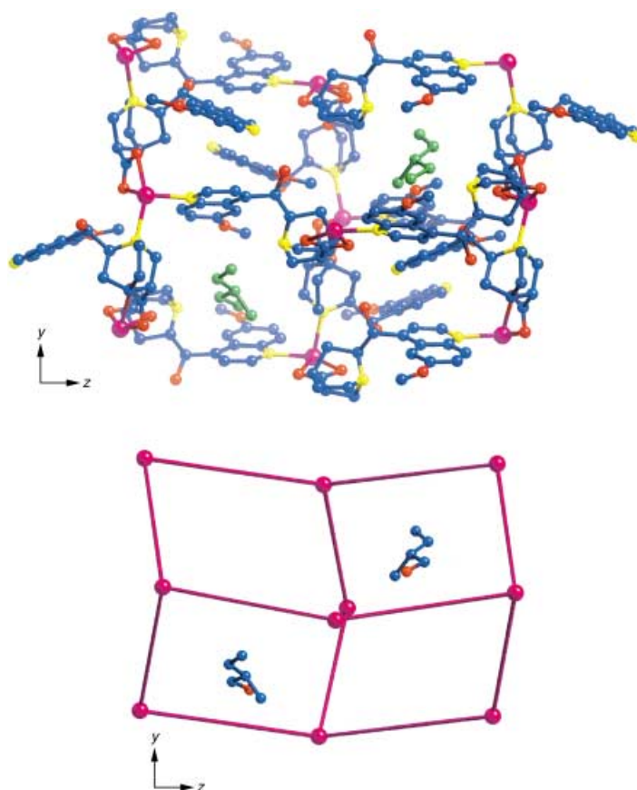
Figure 6. Top: Part of the diamond-like network of 3 including (S)-2-methyl-1-butanol. Bottom: A simplified diamond-like network clearly showing the (S)-2-methyl-1-butanol sites in the chiral cavity.
